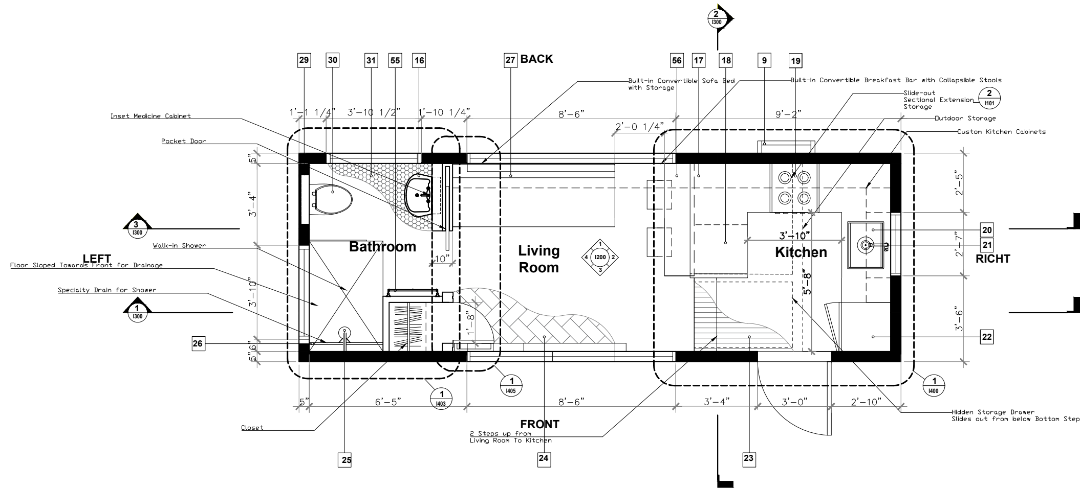
2 FINISH PLAN LEVEL 1 SCALE: 1/4" = 1'-0"
