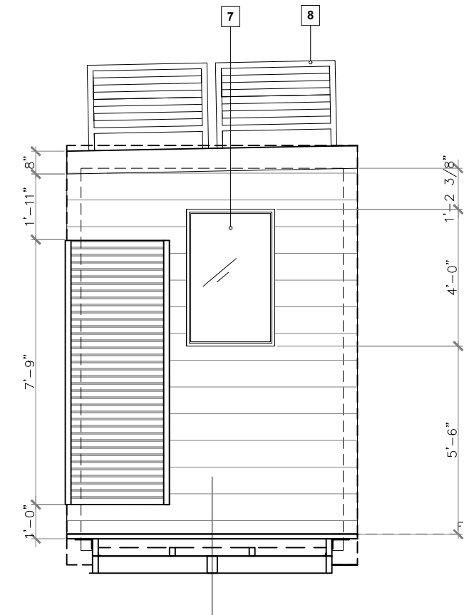
4 SIDE EXTERIOR 1
