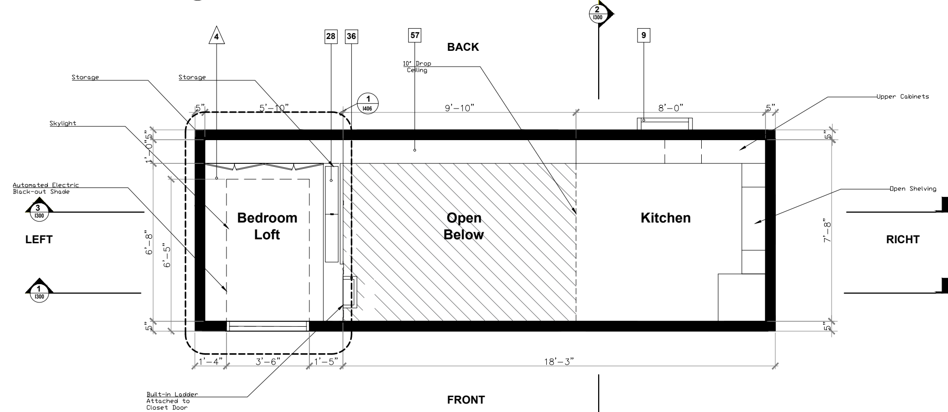
1 FINISH PLAN LEVEL 2 SCALE: 1/4" = 1'-0"
