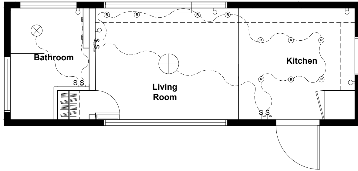
2 ELECTRICAL PLAN LEVEL 1 SCALE: 1/4" = 1'-0"
