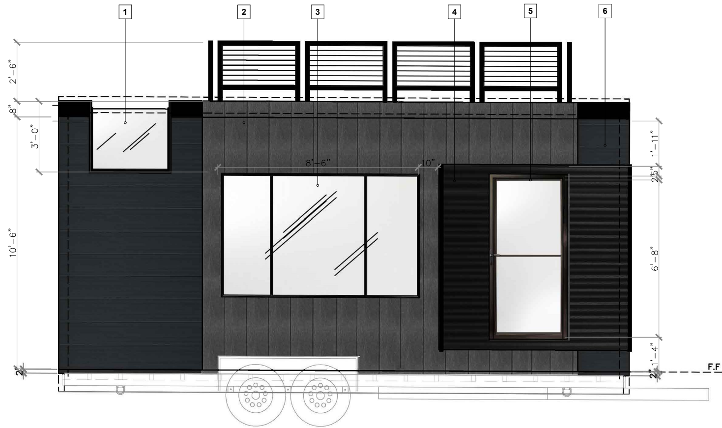
3 FRONT EXTERIOR
