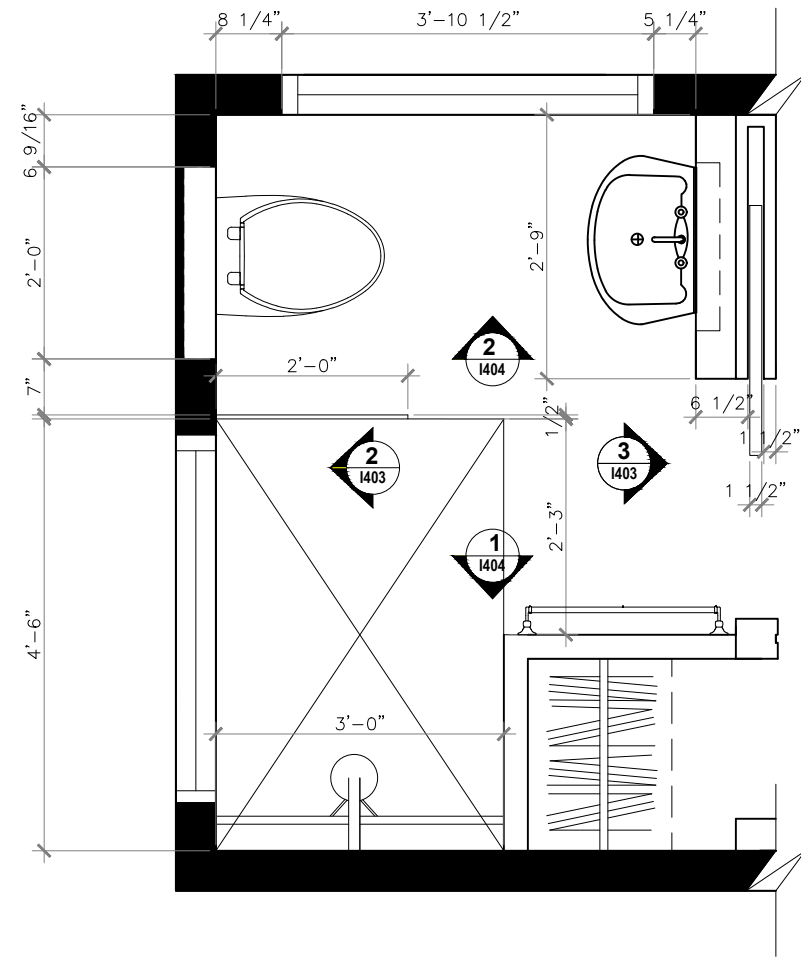
1 ENLARGED BATHROOM PLAN SCALE: 1/4" = 1'-0"
