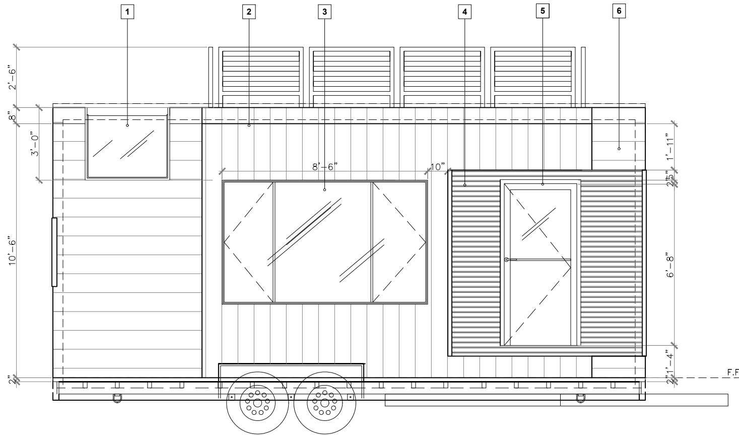
3 FRONT EXTERIOR
