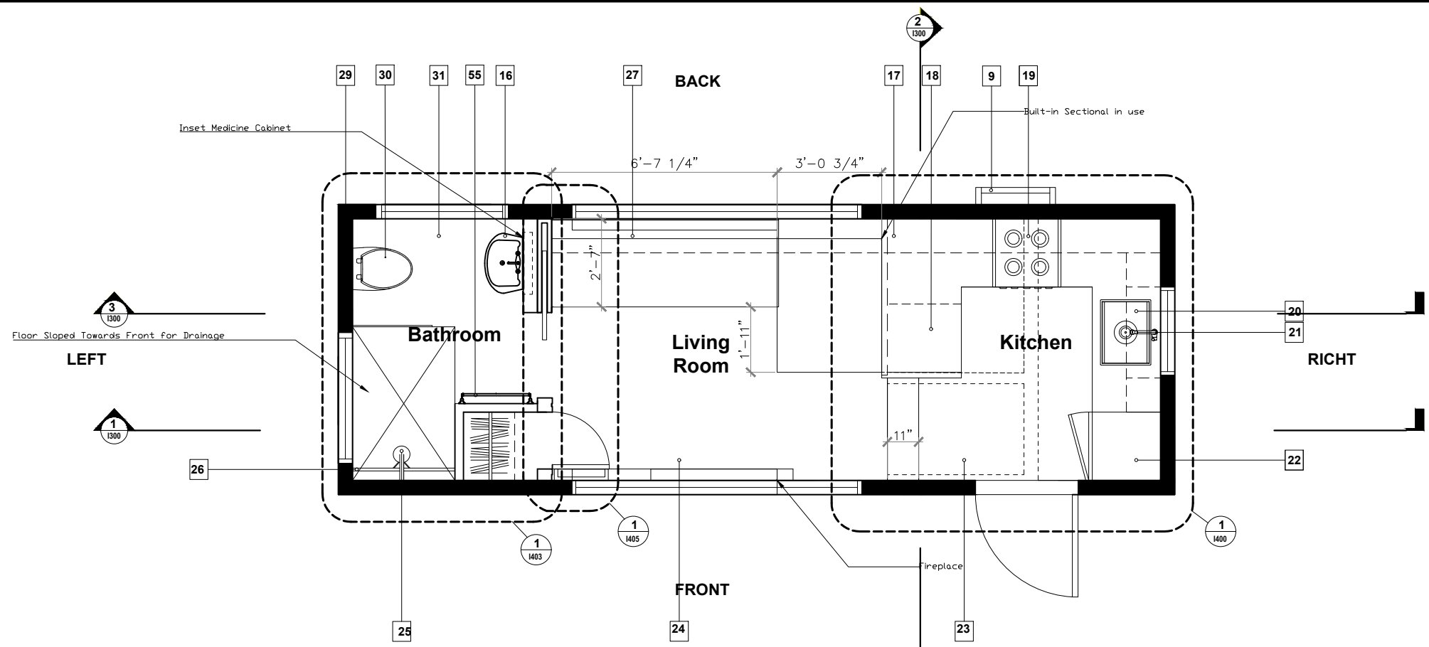
2 FINISH PLAN LEVEL 1 OPTION 2 SCALE: 1/4" = 1'-0"
