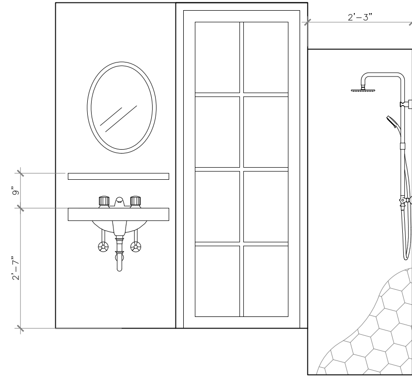
3 ENLARGED BATHROOM ELEVATION SCALE: 1/4" = 1'-0"
