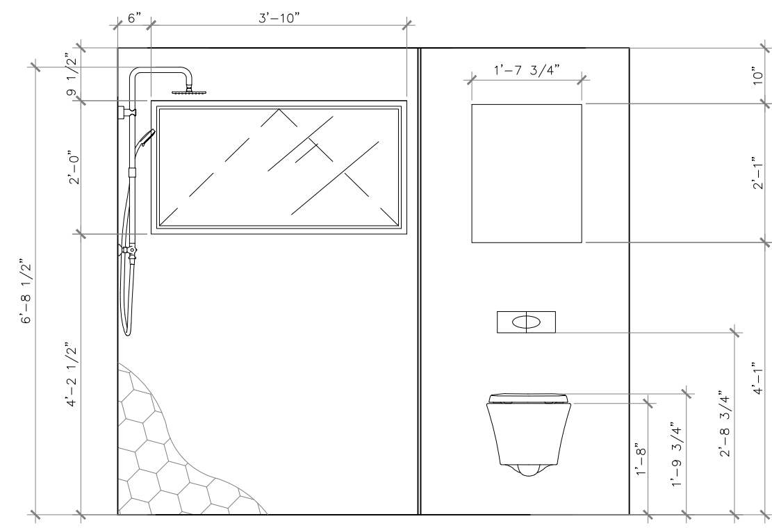
3 ENLARGED BATHROOM ELEVATION SCALE: 1/4" = 1'-0"
